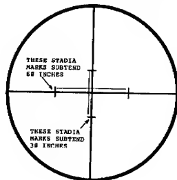
Figure 2-16. ART I reticle.
